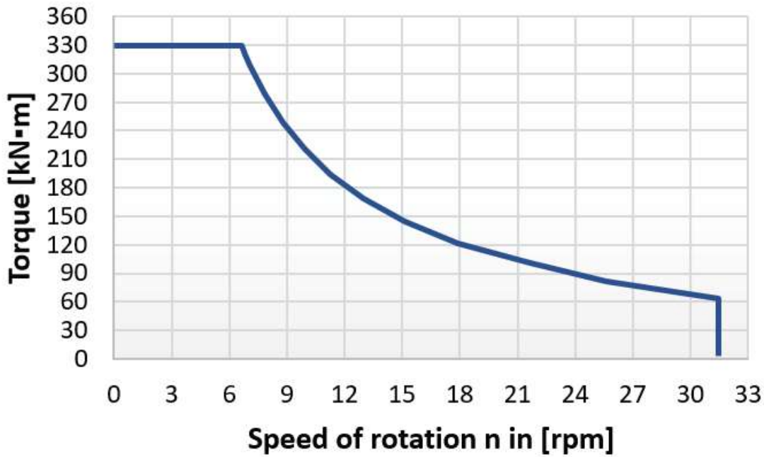
Rotary head
