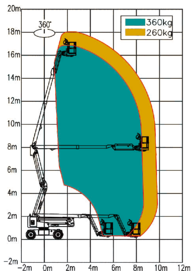
Working rang of SWA18JE-P
