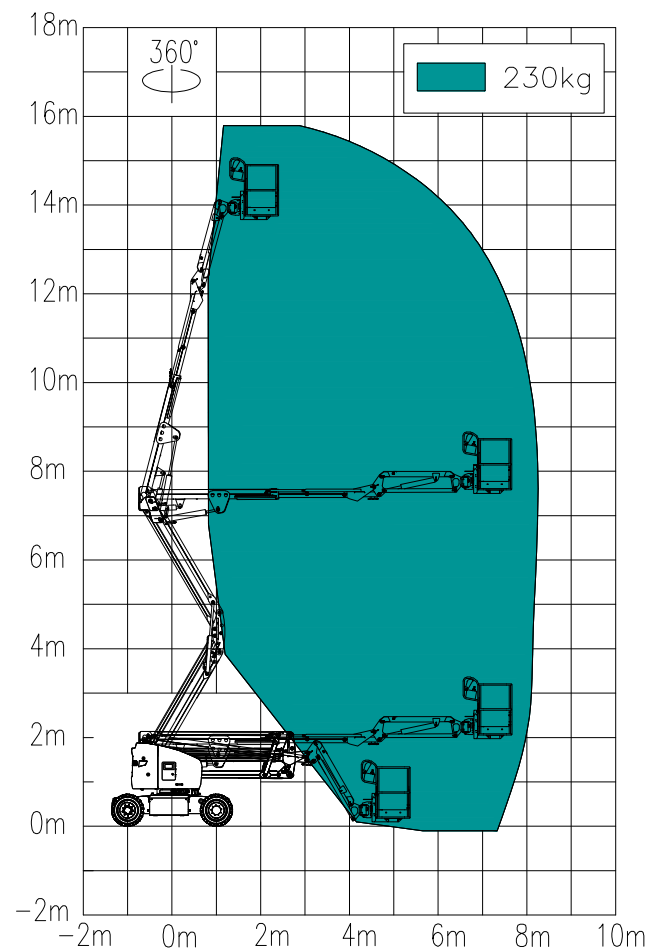
Working range of SWA16JE
