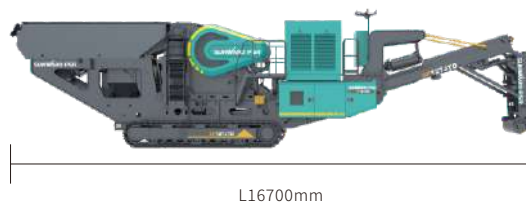
运输尺寸 Transportation Dimension
